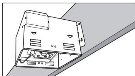
Mounted to L-joists & joists
