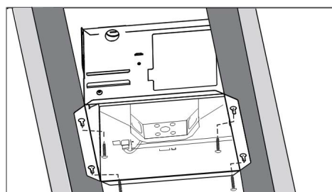
Mounted to L-joists & joists (Available for KCE 100PA, KCE 140PA, KCE 71PD, KCE 140PD and KCE 180PD)
